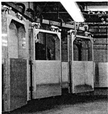
(3) The cans are placed in aluminum boxes that are conveyed into the radiation cell.
