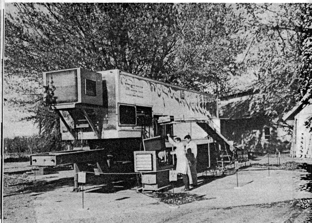
A box of fruit (above the men) moves on a conveyor belt into the Mobile Gamma Irradiator. This device is being used in an orchard to radurize fruit immediately after harvest.
