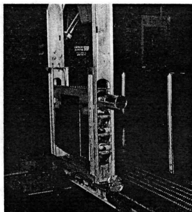
(4) Conveyor racks pass between raised cobalt-60 rods. (See picture on page 16.)
