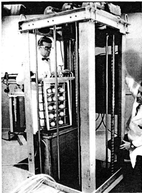
The diagram on the opposite page illustrates the main parts of a research irradiator. Above, scientists load fruit into the research irradiator at the University of California.
