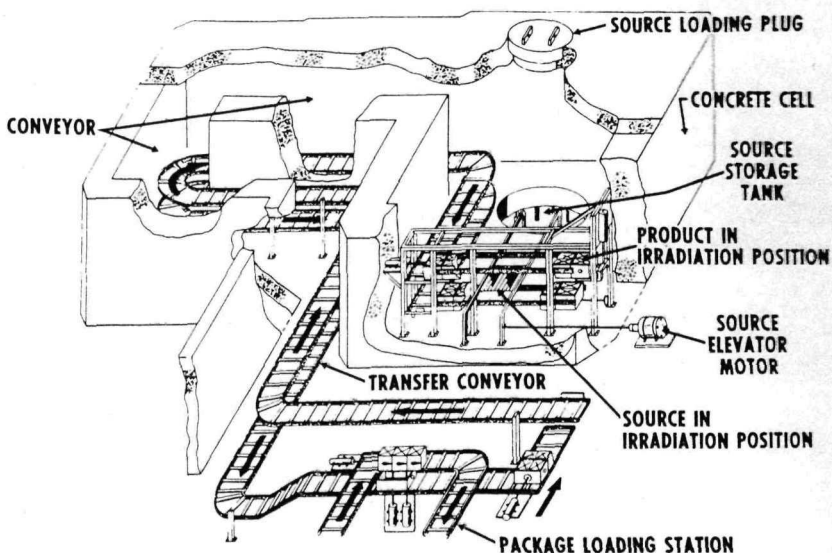
Hawaii Development Irradiator
